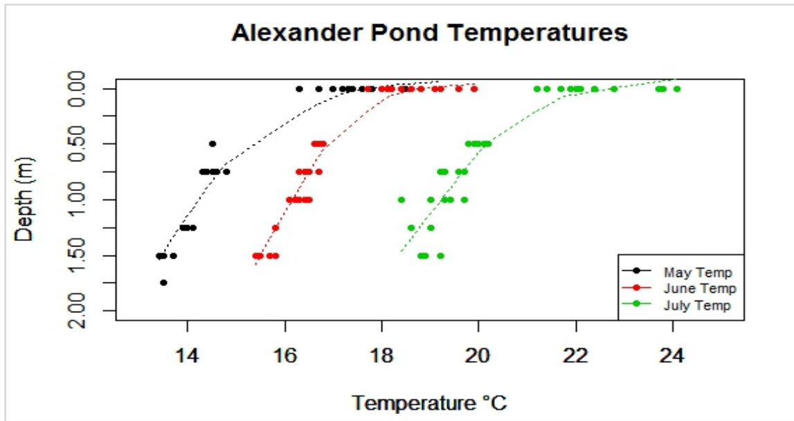
Figure 11. Alexander Pond graph showing temperature variation at various depth readings between May and July 2014. (Krall, raw data 2014).
