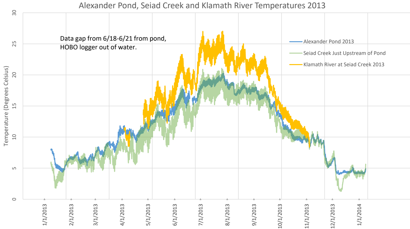
Figure 8. Alexander Pond and Seiad Creek temperatures from HOBO loggers and Klamath River temperatures from the Karuk Water Quality Program's DataSonde for 2013.
